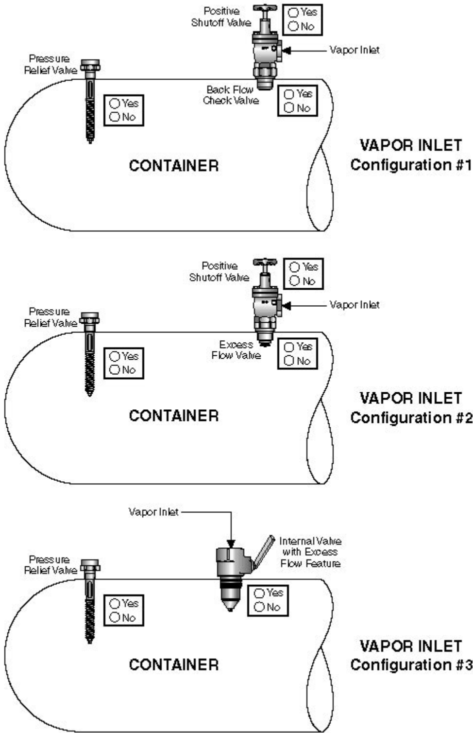
Figure 5-2: Vapor Inlet Appurtenances on Containers of Water Capacity Greater Than 4,000 Gallons
